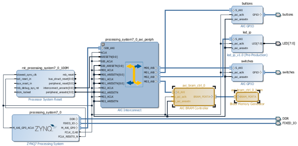
Figure 17. Completed Block Diagram
